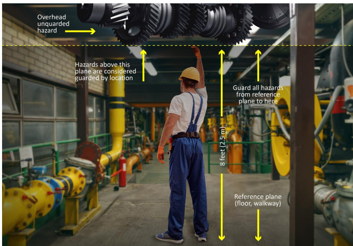
Fig 25: Safeguarding by location and distance
