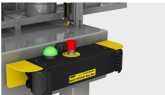
Fig 37: Two-hand control
